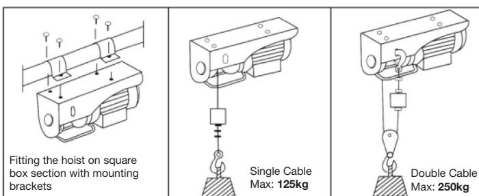
Fig.3 Installation
